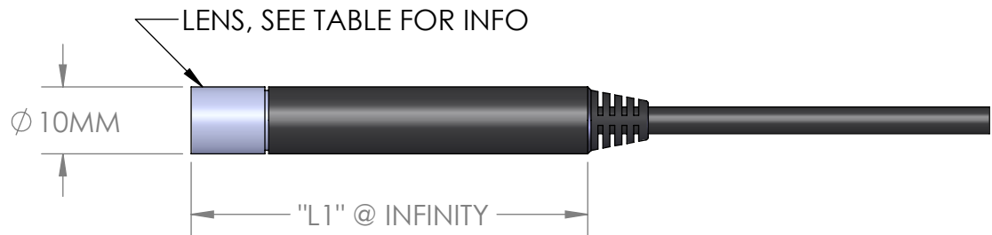
10MM 1/4" CCD CAMERA WITH LENS
